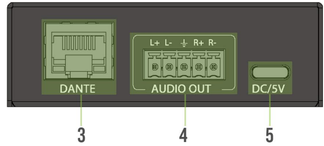
Rear Panel
