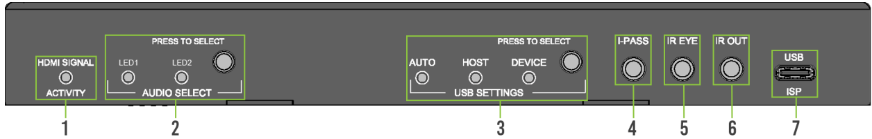
AC-EX40-444-PLUS-R2 (Receiver) – Rear Panel
