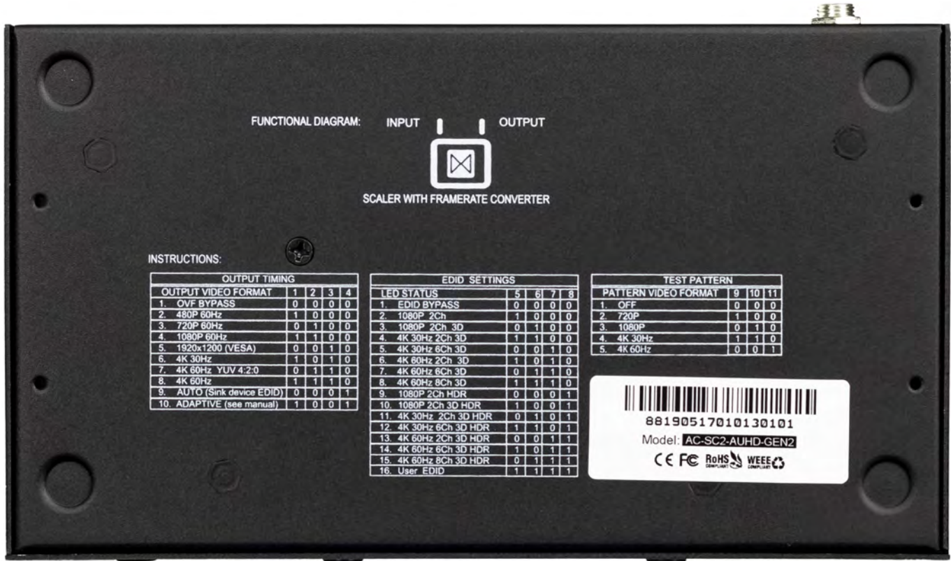
Bottom View
